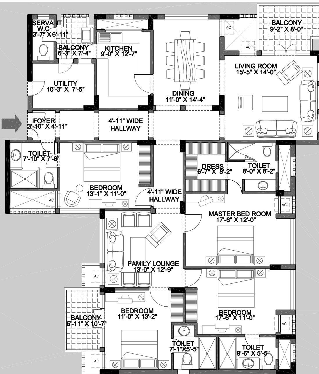
TYPICAL UNIT C - EVEN FLOOR PLAN GARDEN HEIGHTS-1
